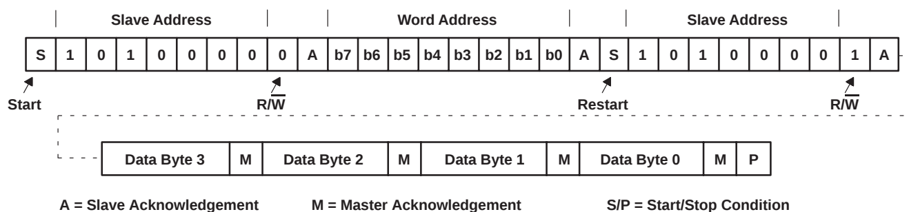
Figure 3-13. EEPROM Interface Doubleword Data Collection
